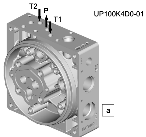
Example of standard circuit UP100K4D0-01
