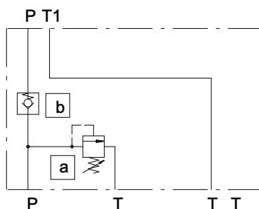
Example of standard circuit UP100K4D0-02
